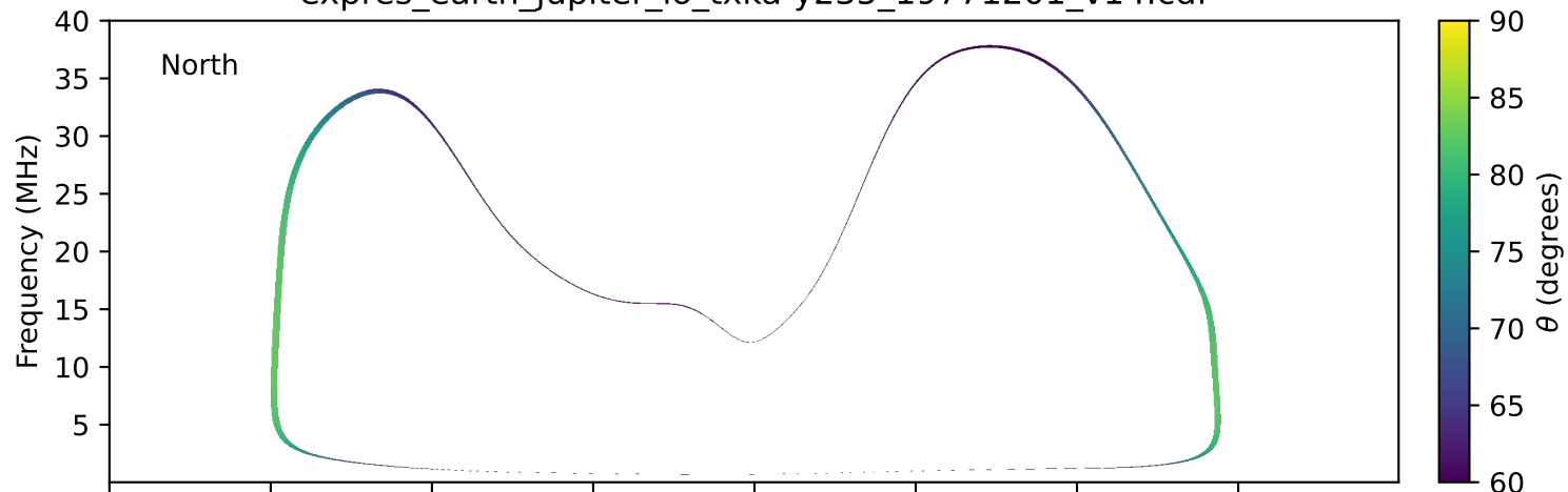
expres_earth_jupiter_io_txka-y235_19771201_v14.cdf
