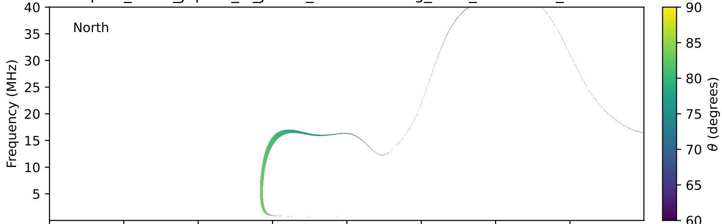
expres_earth_jupiter_io_jrm33_lossc-wid1deg_3kev_19771229_v11.cdf
