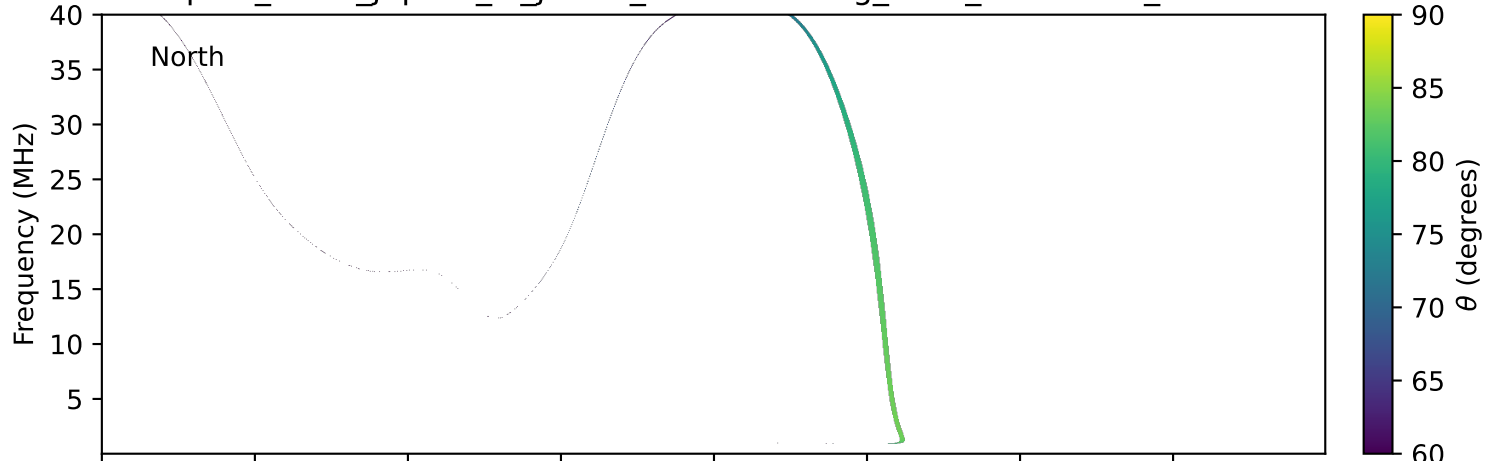
expres_earth_jupiter_io_jrm33_lossc-wid1deg_3kev_19771226_v11.cdf
