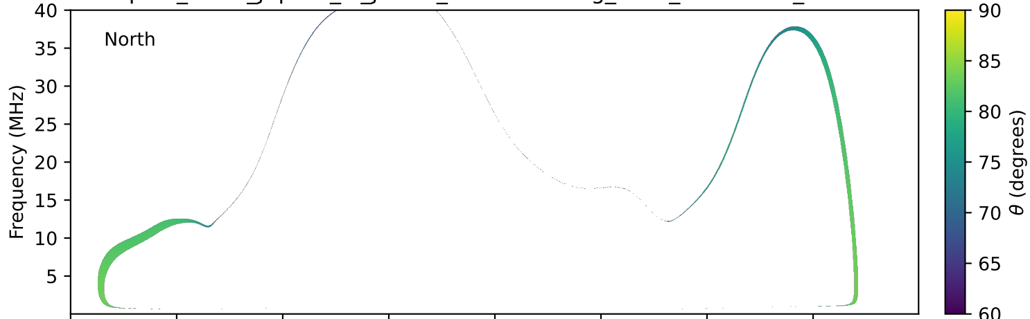
expres_earth_jupiter_io_jrm33_lossc-wid1deg_3kev_19771224_v11.cdf
