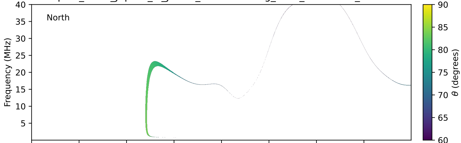
expres_earth_jupiter_io_jrm33_lossc-wid1deg_3kev_19771222_v11.cdf
