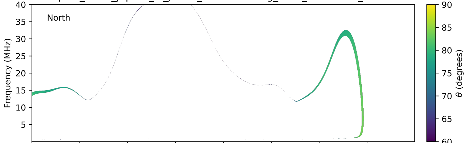
expres_earth_jupiter_io_jrm33_lossc-wid1deg_3kev_19771217_v11.cdf
