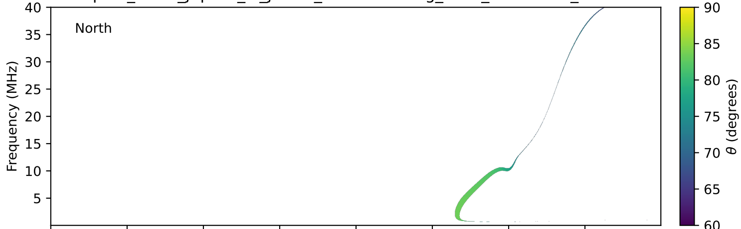
expres_earth_jupiter_io_jrm33_lossc-wid1deg_3kev_19771211_v11.cdf
