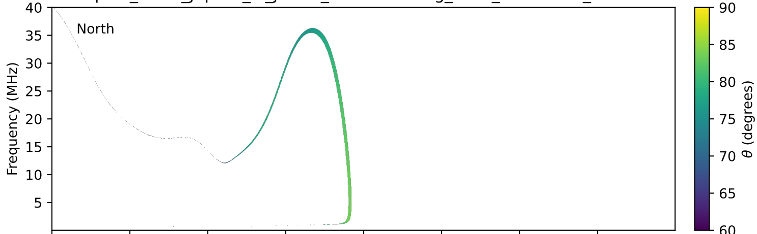
expres_earth_jupiter_io_jrm33_lossc-wid1deg_3kev_19771205_v11.cdf
