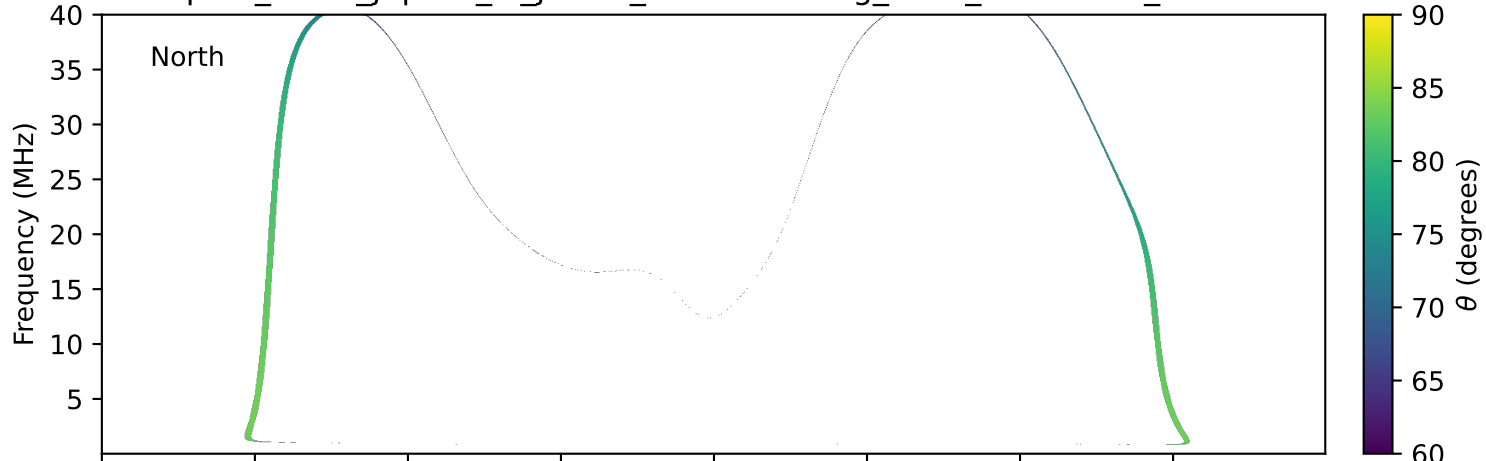
expres_earth_jupiter_io_jrm33_lossc-wid1deg_3kev_19771201_v11.cdf
