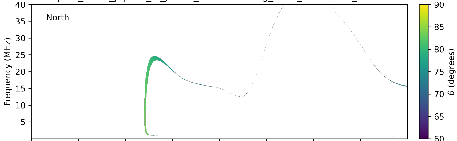
expres_earth_jupiter_io_jrm09_lossc-wid1deg_3kev_19771222_v11.cdf
