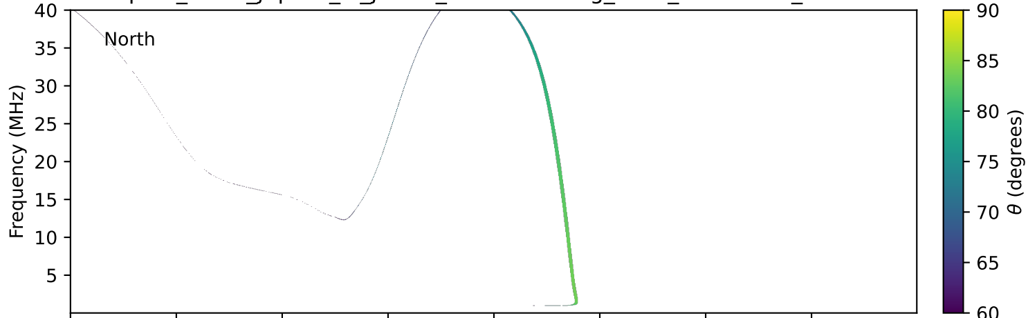
expres_earth_jupiter_io_jrm09_lossc-wid1deg_3kev_19771219_v11.cdf
