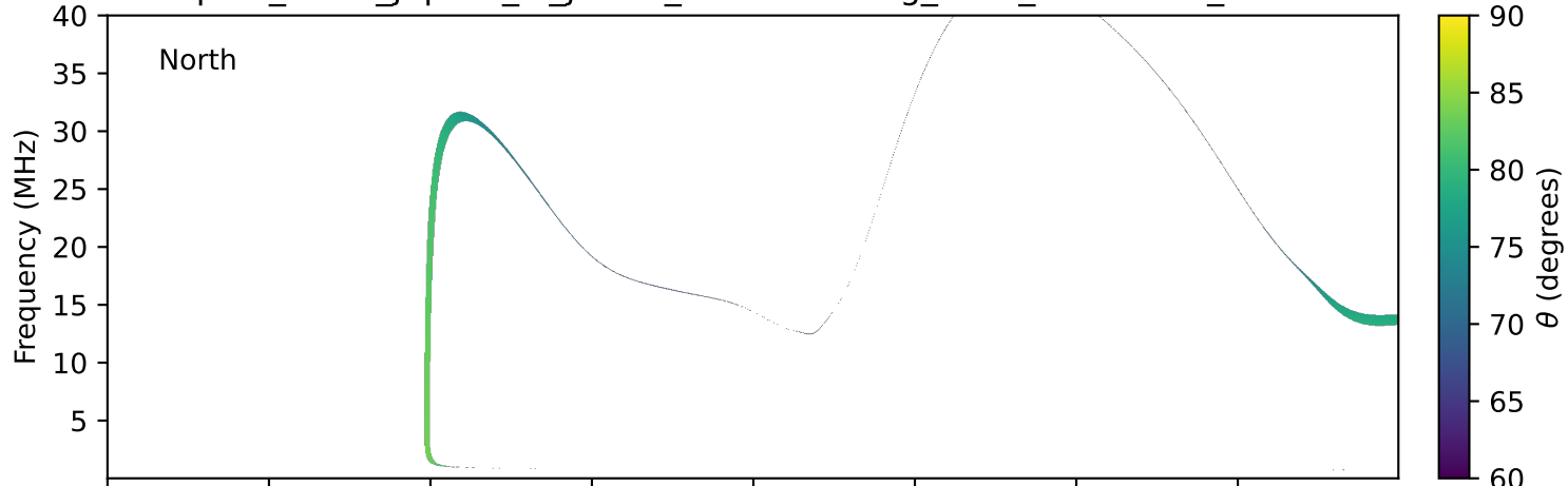
expres_earth_jupiter_io_jrm09_lossc-wid1deg_3kev_19771215_v11.cdf
