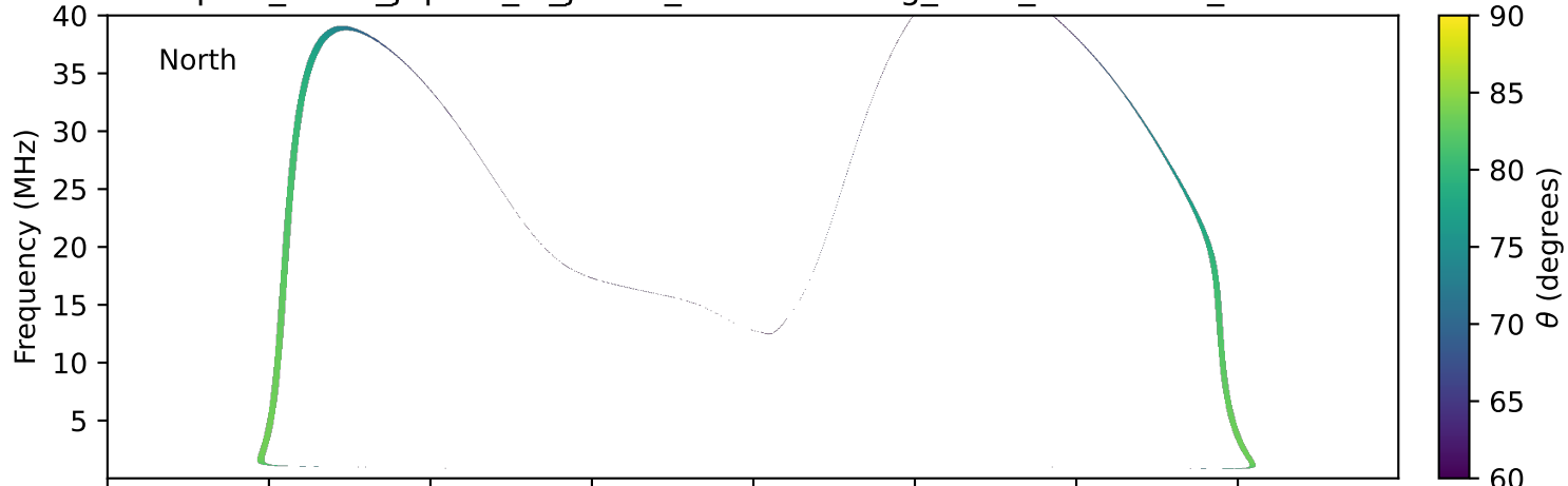
expres_earth_jupiter_io_jrm09_lossc-wid1deg_3kev_19771201_v11.cdf
