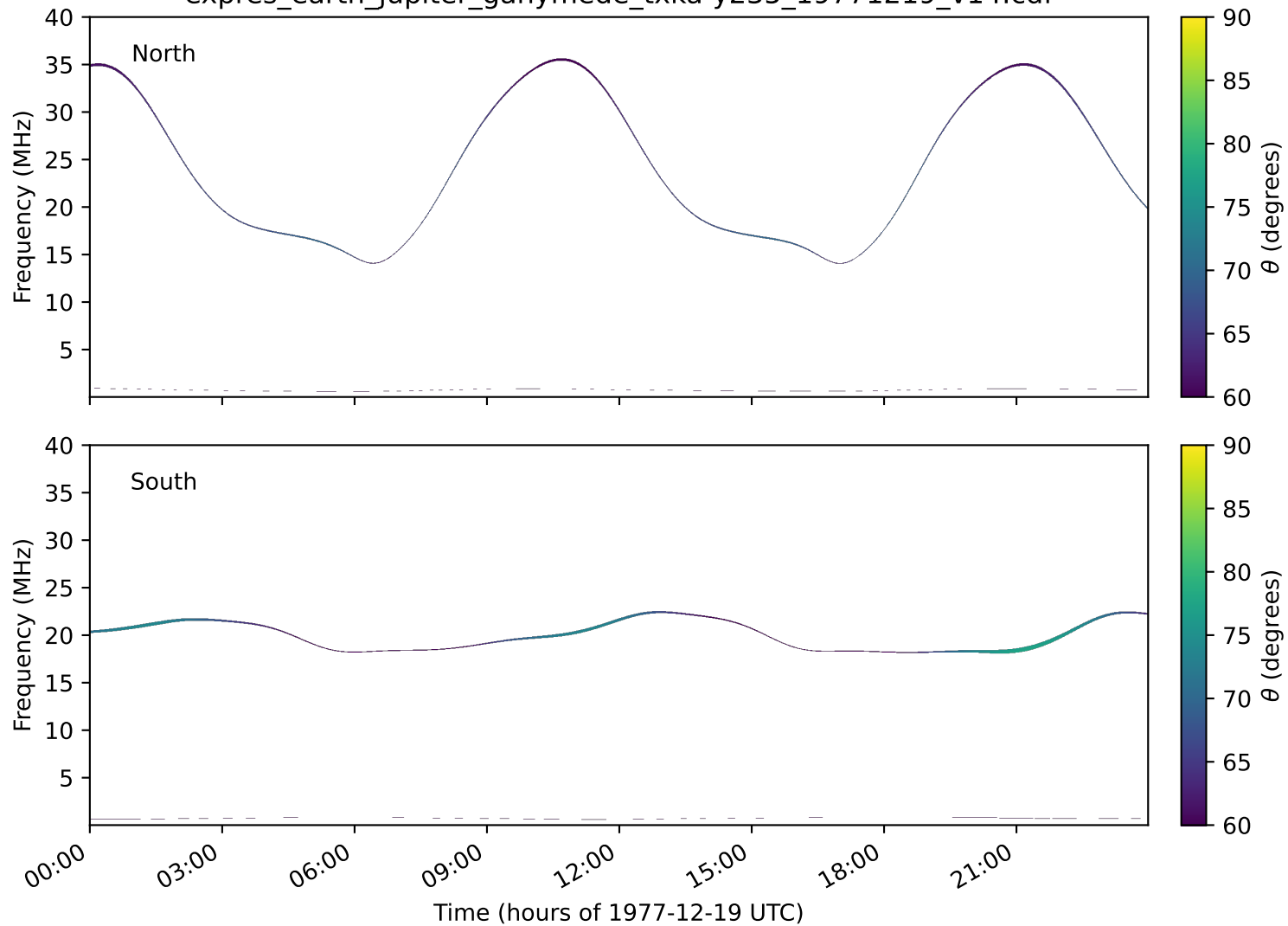
expres_earth_jupiter_ganymede_txka-y235_19771219_v14.cdf
