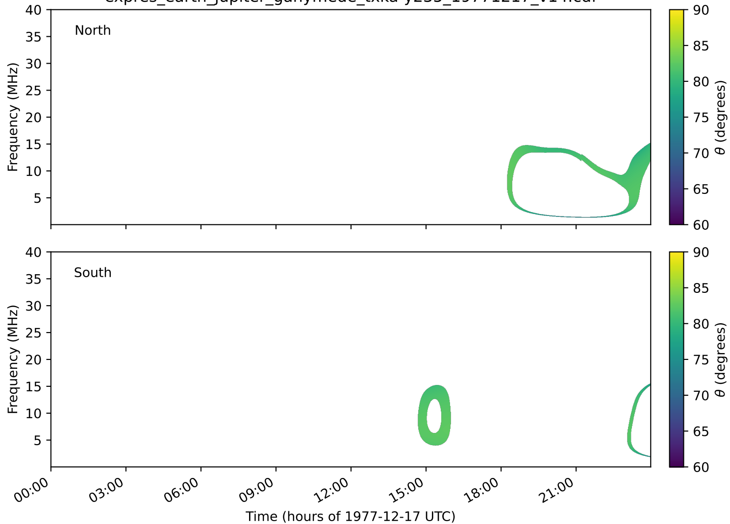
expres_earth_jupiter_ganymede_txka-y235_19771217_v14.cdf
