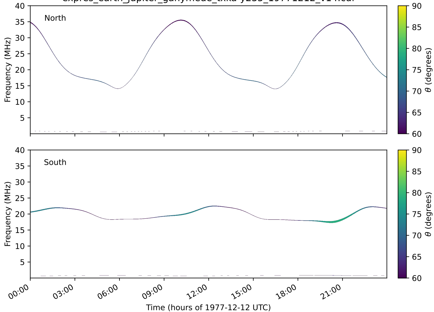
expres_earth_jupiter_ganymede_txka-y235_19771212_v14.cdf
