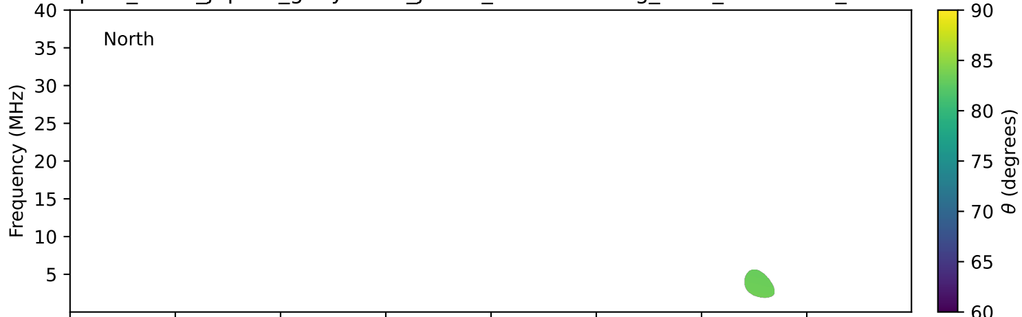
expres_earth_jupiter_ganymede_jrm09_lossc-wid1deg_3kev_19771217_v11.cdf
