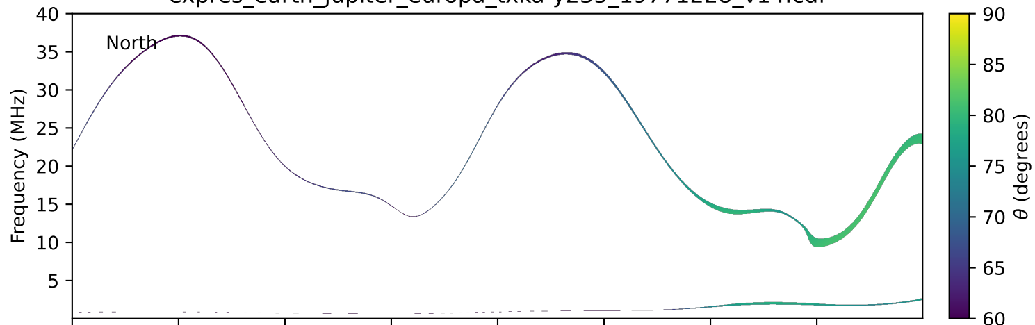
expres_earth_jupiter_europa_txka-y235_19771228_v14.cdf
