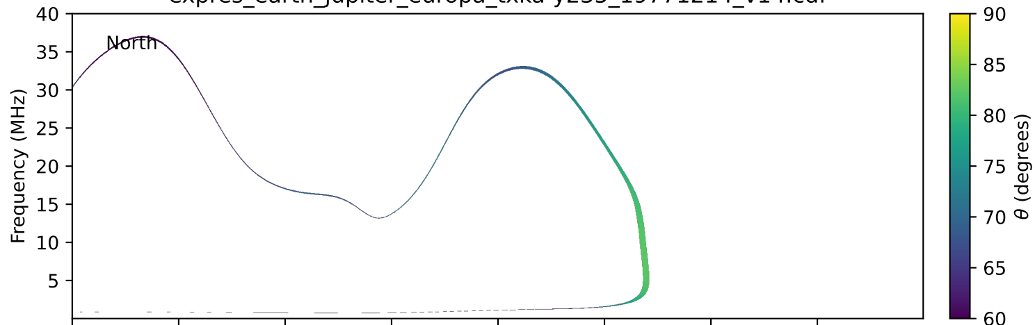
expres_earth_jupiter_europa_txka-y235_19771214_v14.cdf
