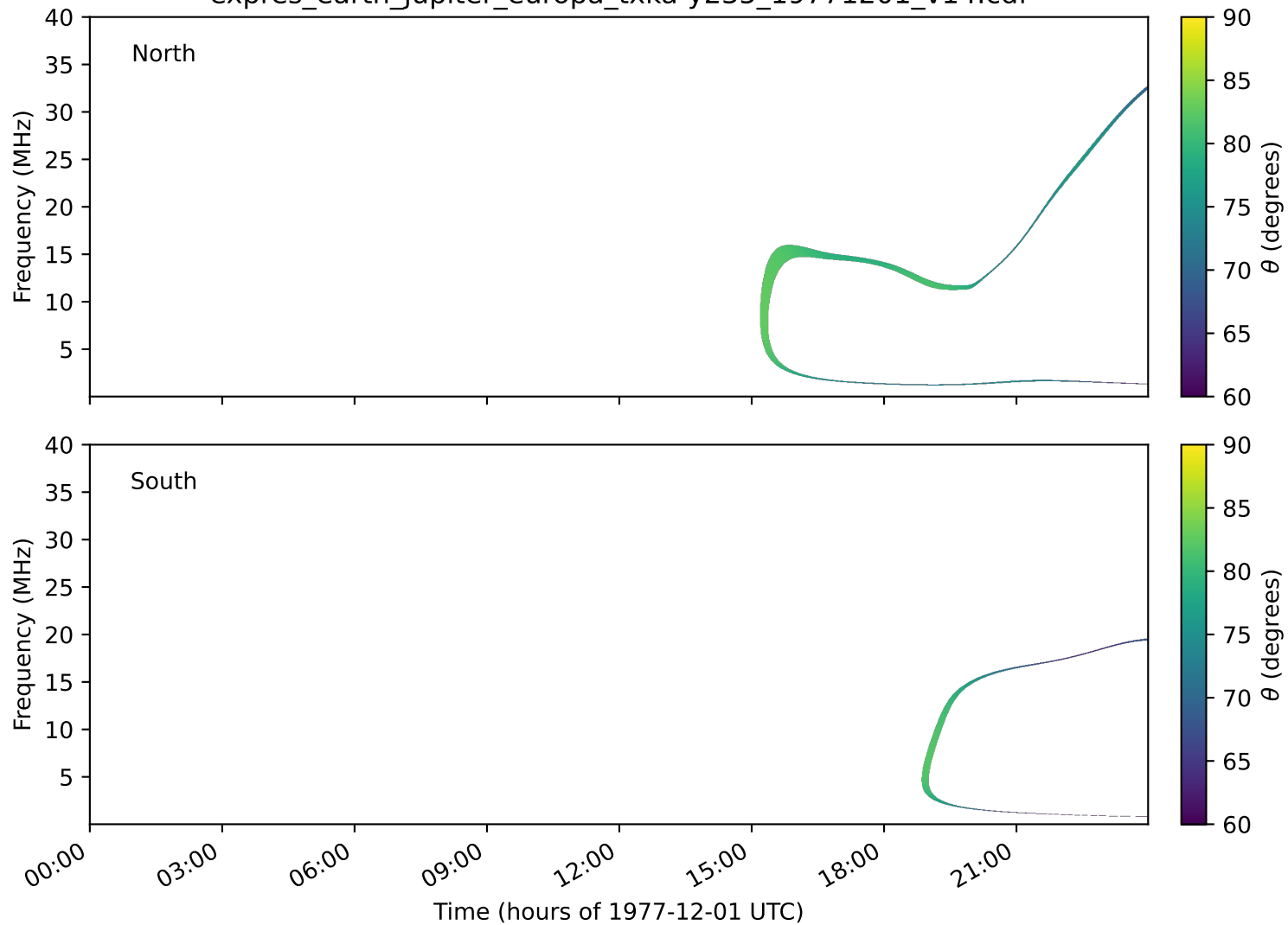
expres_earth_jupiter_europa_txka-y235_19771201_v14.cdf
