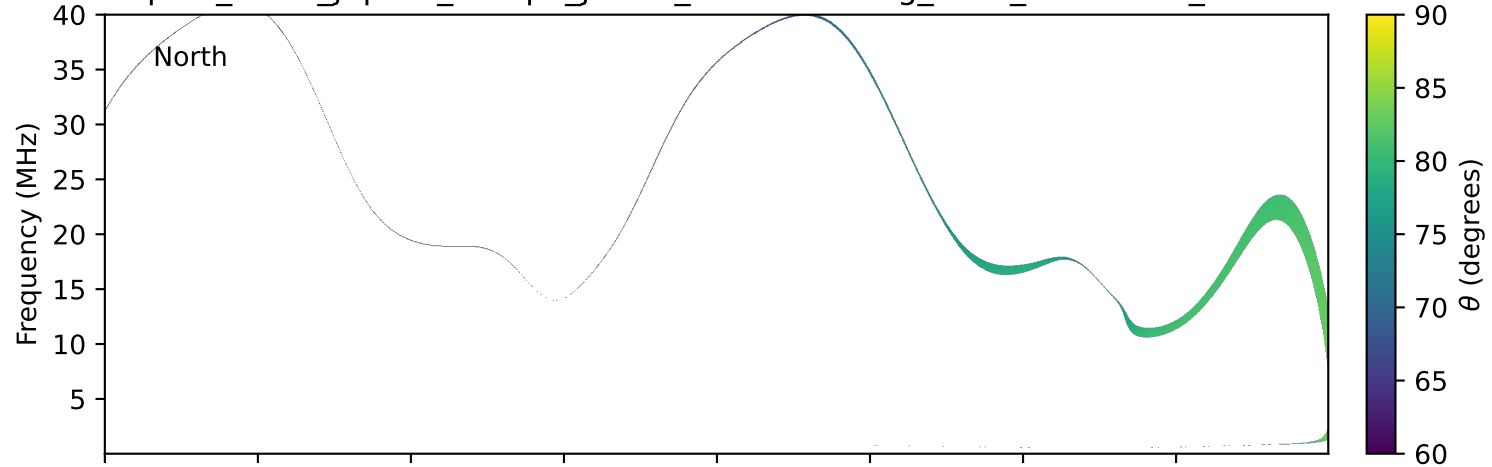
expres_earth_jupiter_europa_jrm33_lossc-wid1deg_3kev_19771221_v11.cdf
