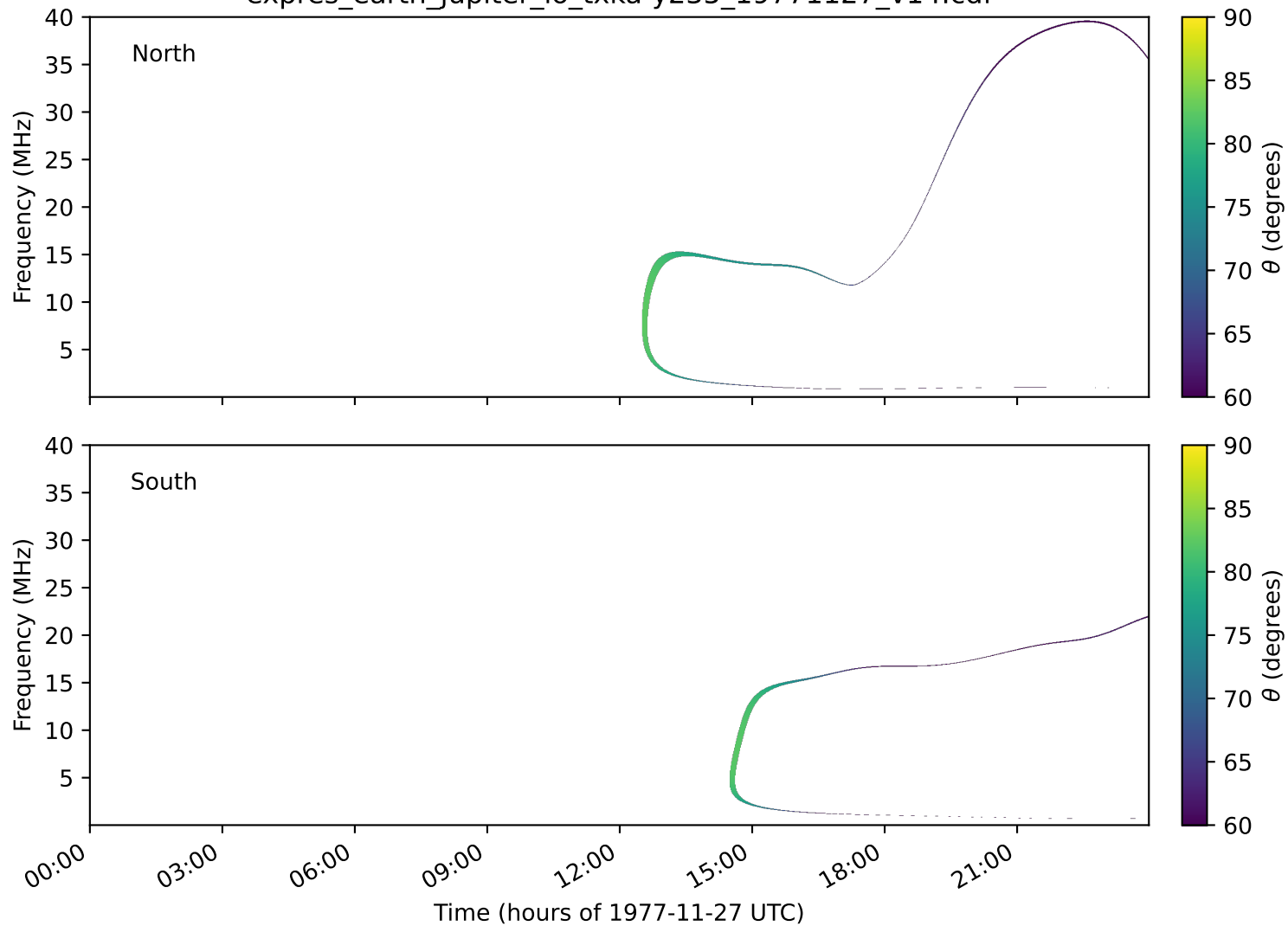
expres_earth_jupiter_io_txka-y235_19771127_v14.cdf
