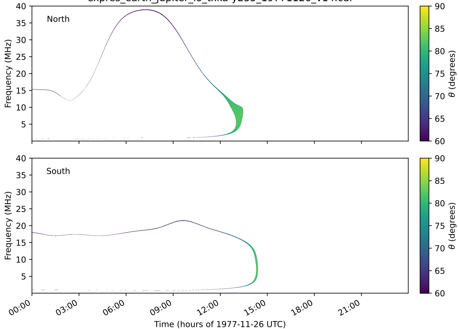
expres_earth_jupiter_io_txka-y235_19771126_v14.cdf
