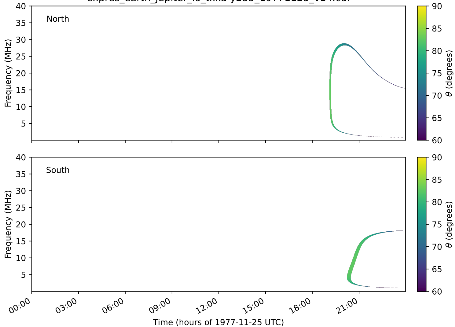
expres_earth_jupiter_io_txka-y235_19771125_v14.cdf
