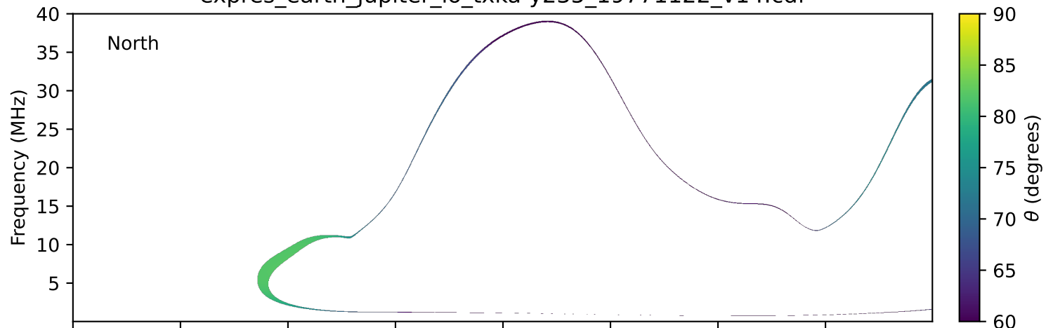
expres_earth_jupiter_io_txka-y235_19771122_v14.cdf
