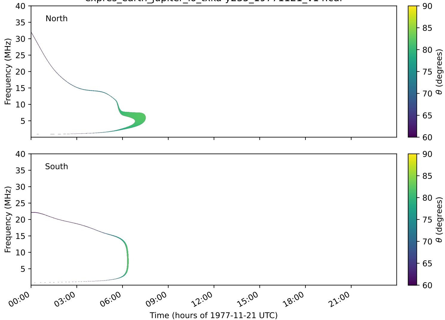
expres_earth_jupiter_io_txka-y235_19771121_v14.cdf
