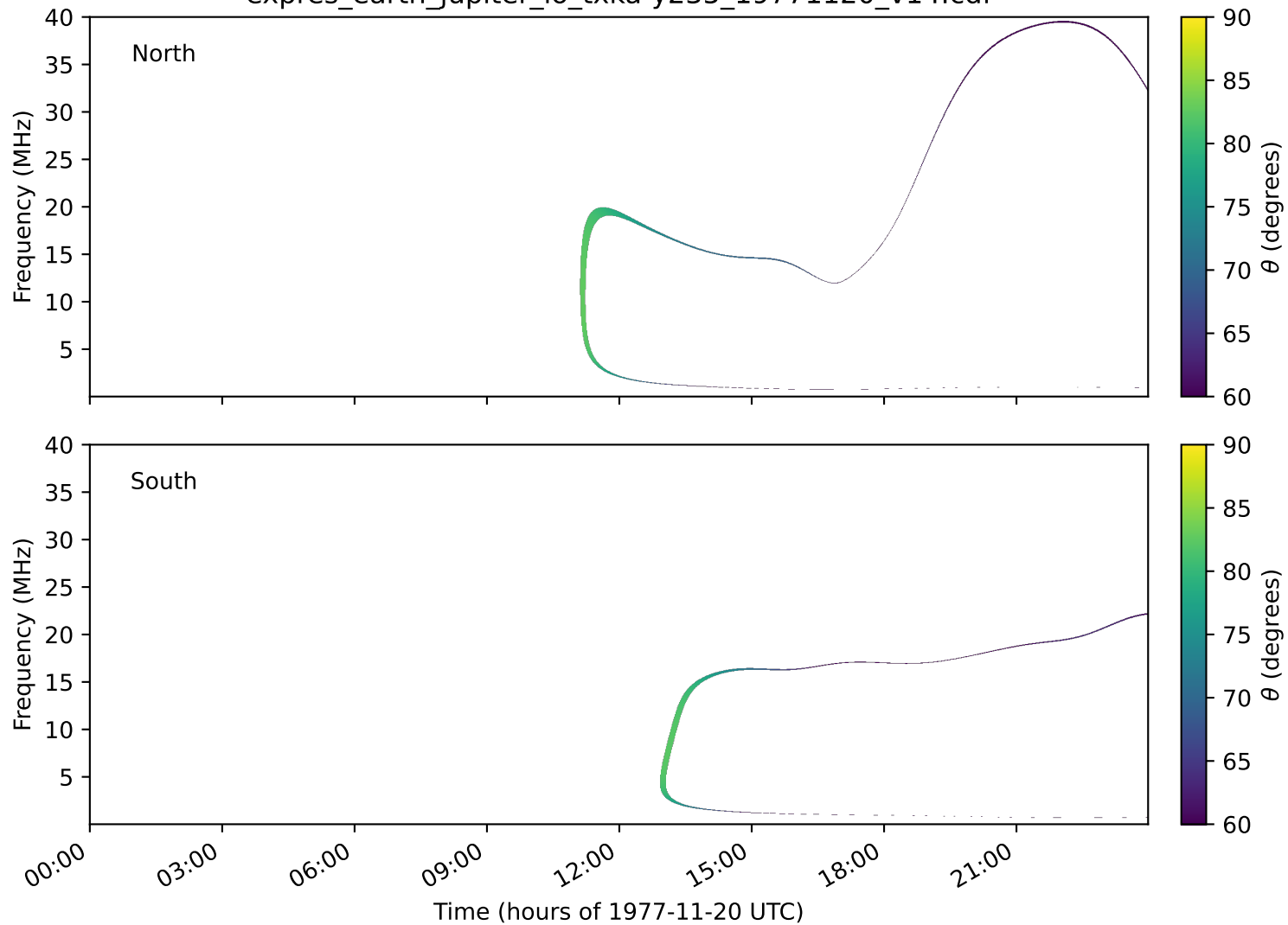
expres_earth_jupiter_io_txka-y235_19771120_v14.cdf
