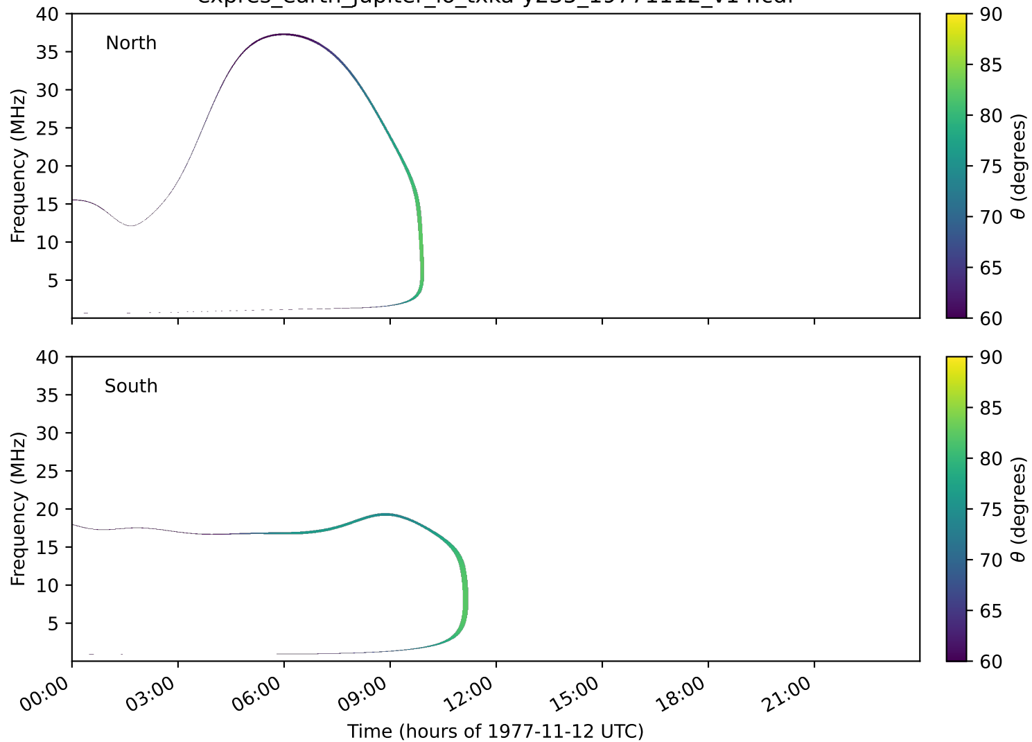
expres_earth_jupiter_io_txka-y235_19771112_v14.cdf
