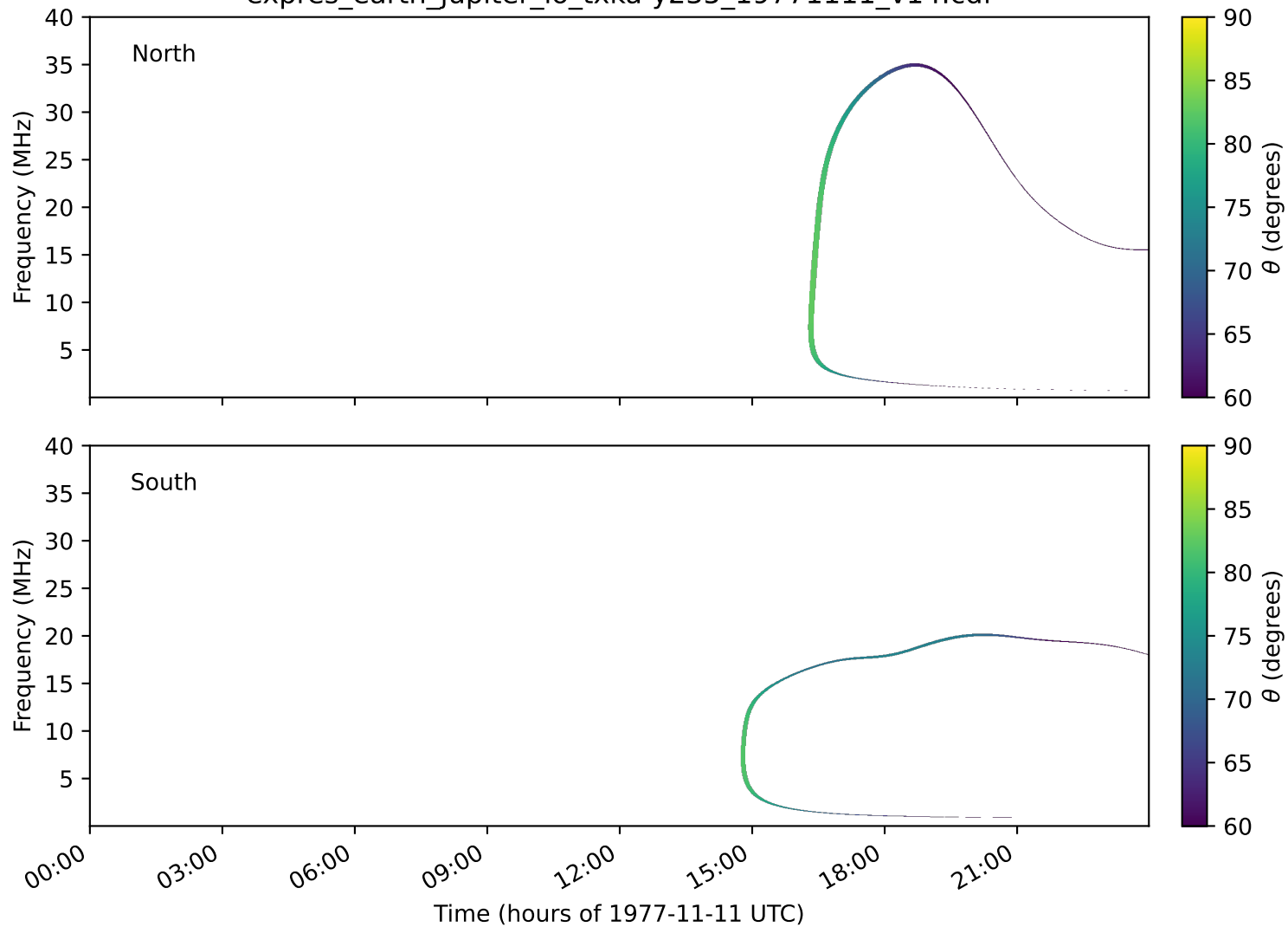
expres_earth_jupiter_io_txka-y235_19771111_v14.cdf
