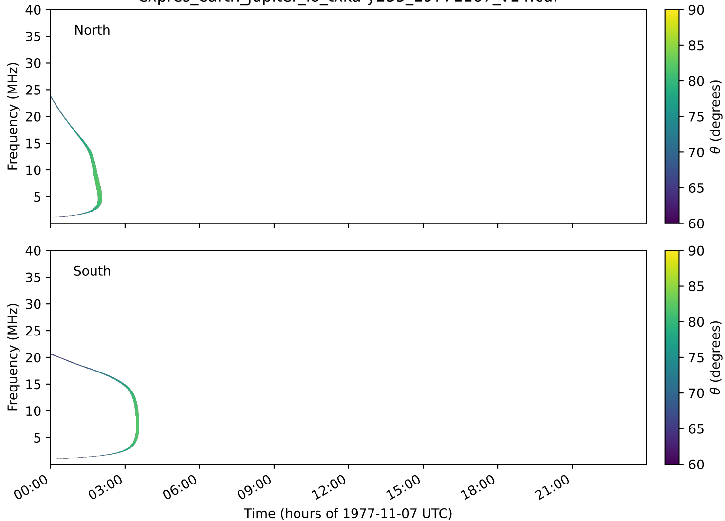
expres_earth_jupiter_io_txka-y235_19771107_v14.cdf
