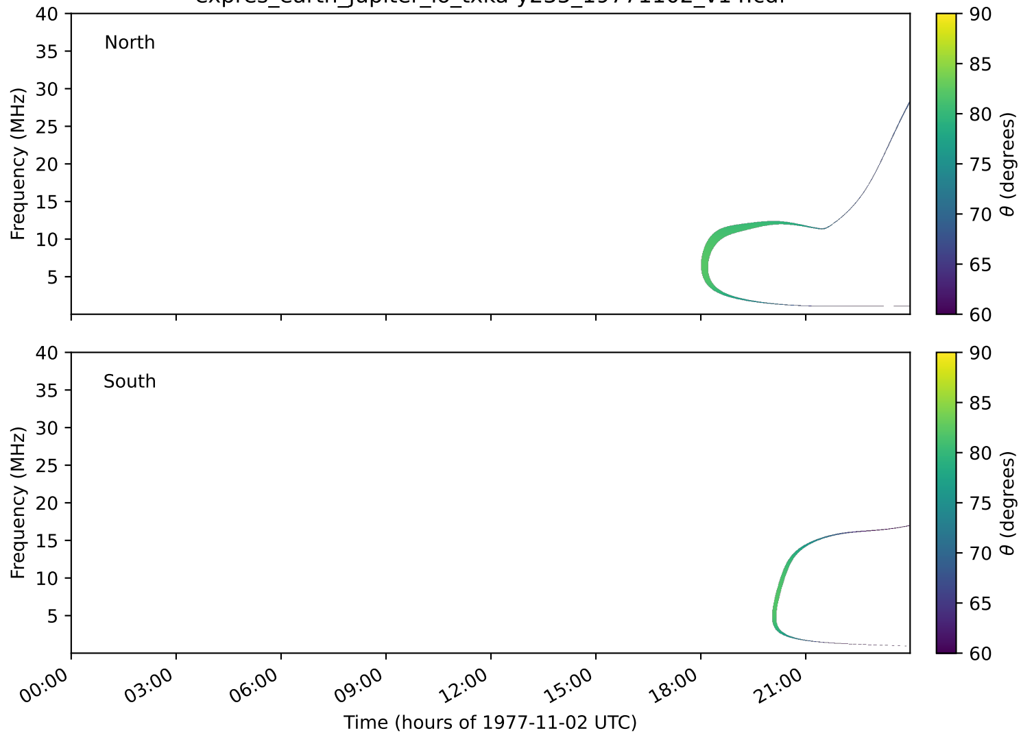
expres_earth_jupiter_io_txka-y235_19771102_v14.cdf
