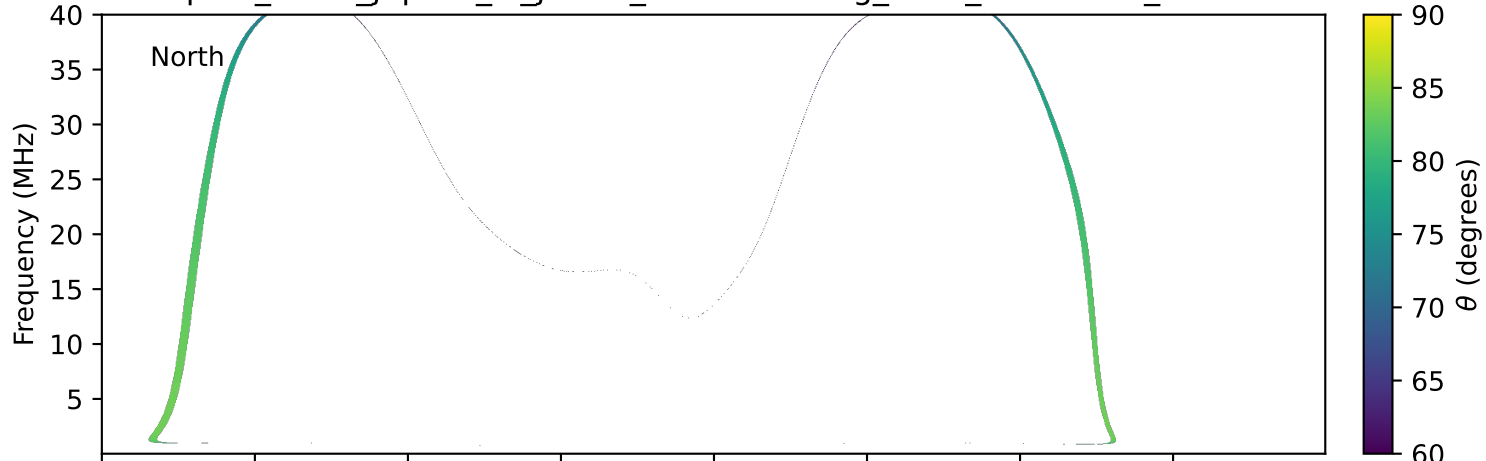
expres_earth_jupiter_io_jrm33_lossc-wid1deg_3kev_19771124_v11.cdf
