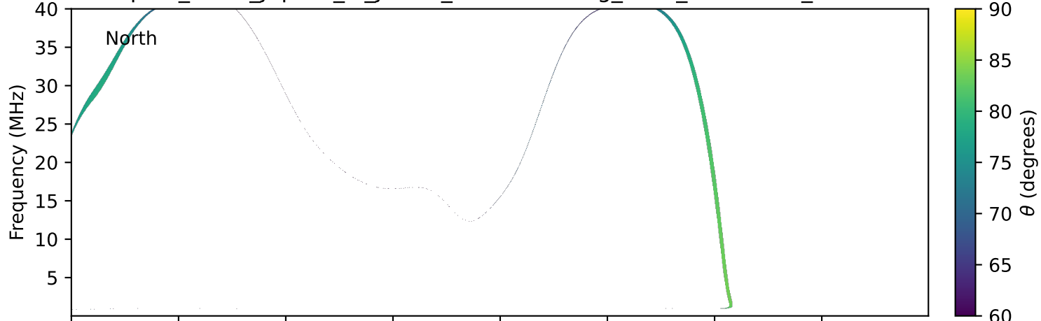
expres_earth_jupiter_io_jrm33_lossc-wid1deg_3kev_19771117_v11.cdf
