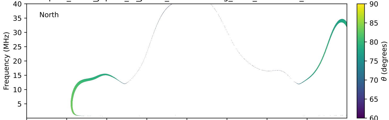
expres_earth_jupiter_io_jrm33_lossc-wid1deg_3kev_19771115_v11.cdf
