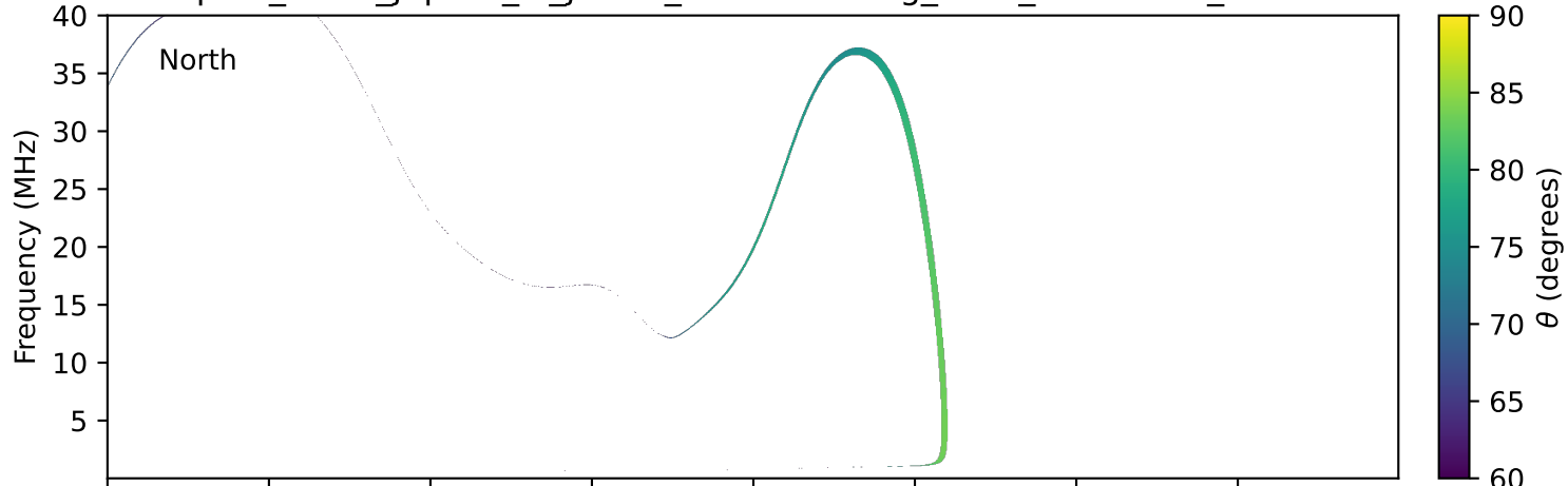
expres_earth_jupiter_io_jrm33_lossc-wid1deg_3kev_19771103_v11.cdf
