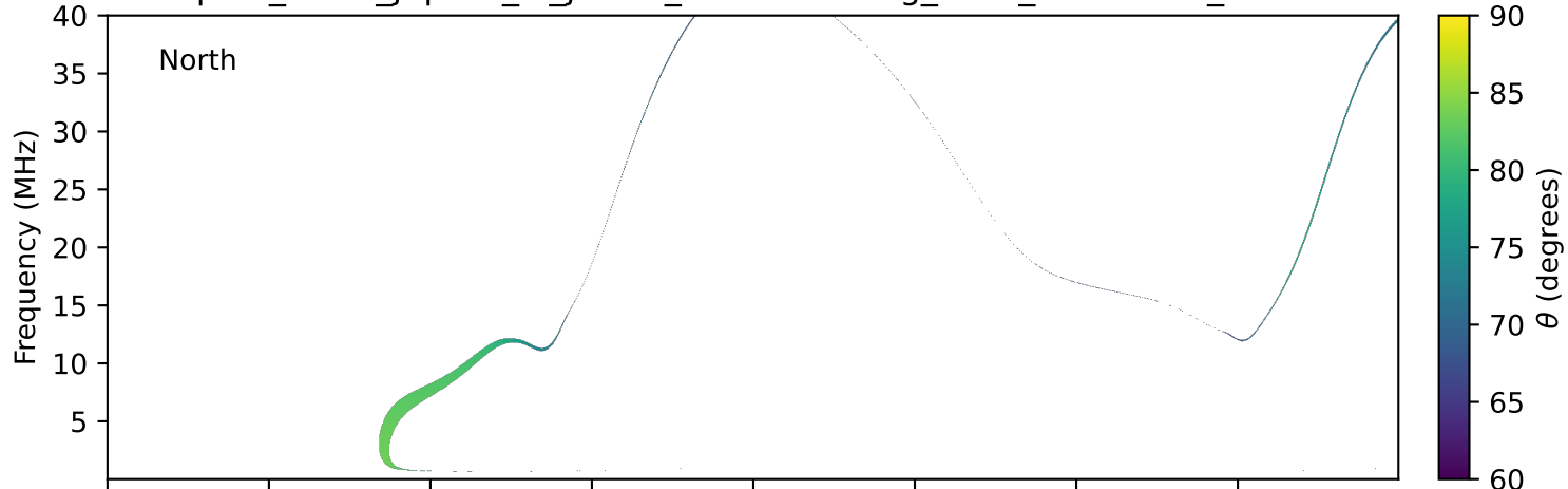
expres_earth_jupiter_io_jrm09_lossc-wid1deg_3kev_19771122_v11.cdf
