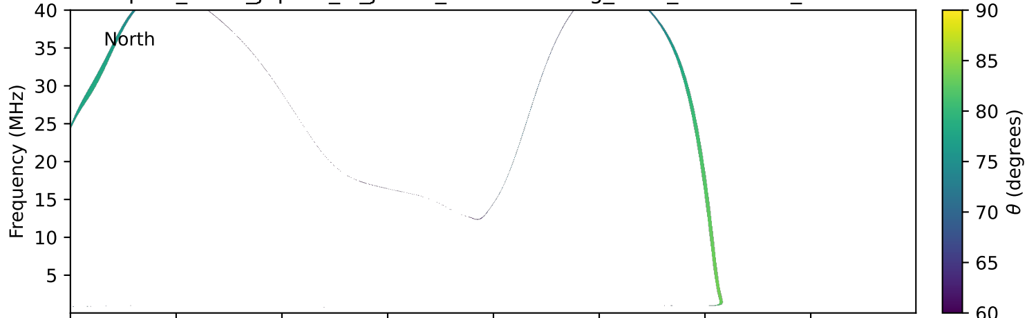
expres_earth_jupiter_io_jrm09_lossc-wid1deg_3kev_19771117_v11.cdf
