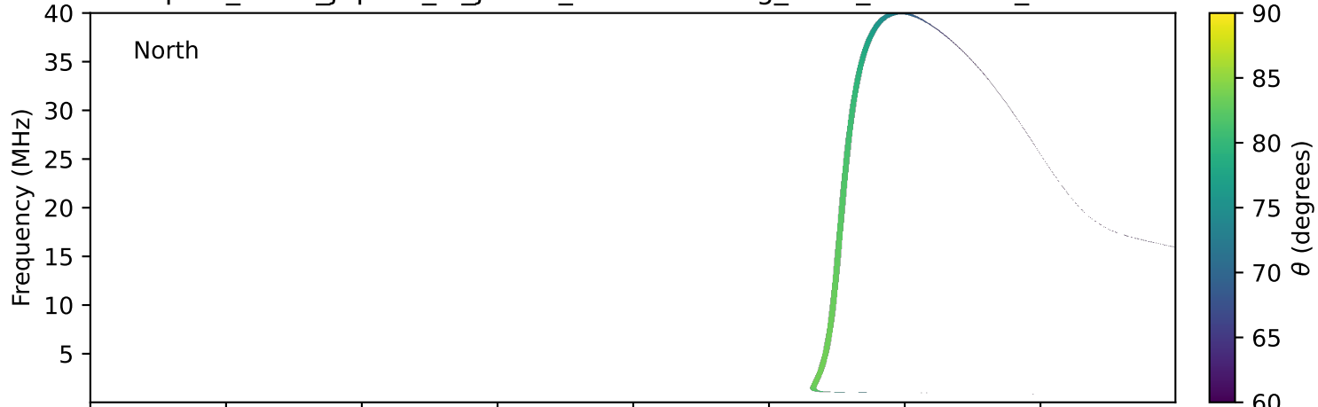
expres_earth_jupiter_io_jrm09_lossc-wid1deg_3kev_19771111_v11.cdf
