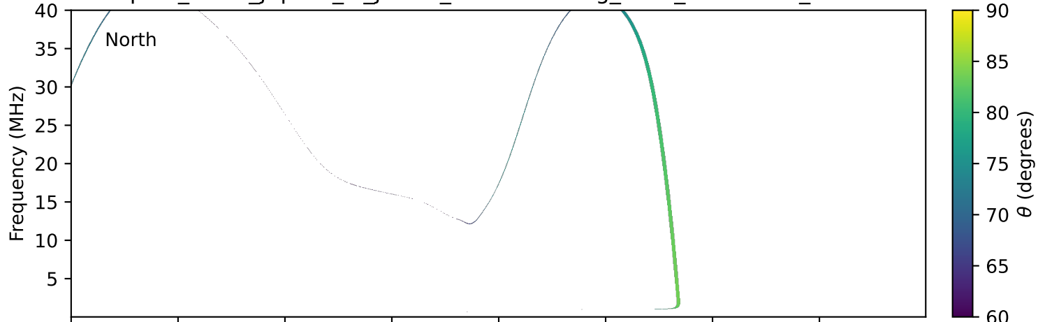
expres_earth_jupiter_io_jrm09_lossc-wid1deg_3kev_19771110_v11.cdf
