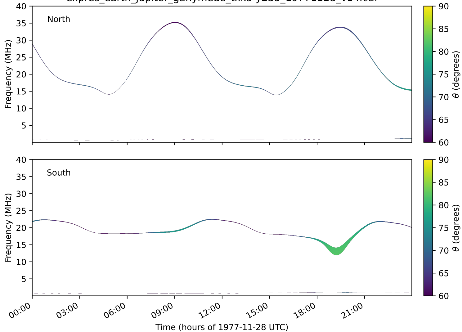
expres_earth_jupiter_ganymede_txka-y235_19771128_v14.cdf
