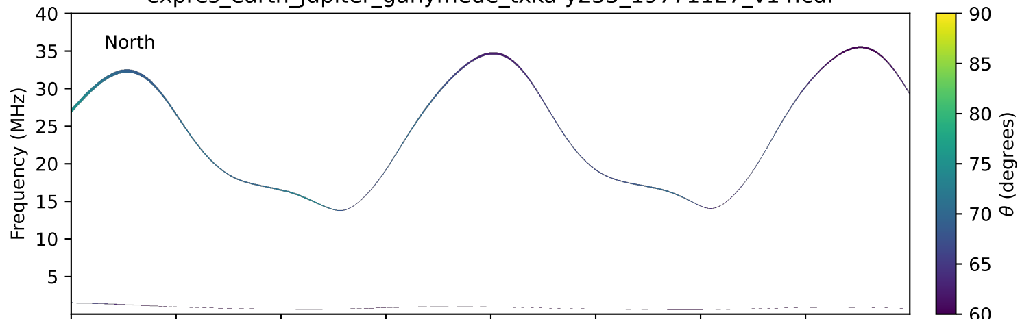
expres_earth_jupiter_ganymede_txka-y235_19771127_v14.cdf
