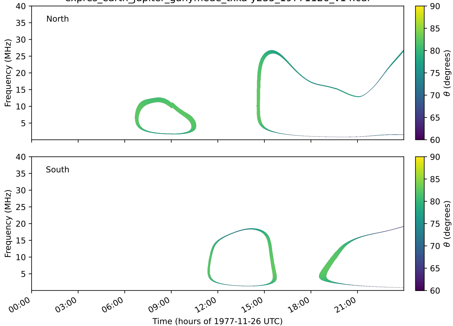
expres_earth_jupiter_ganymede_txka-y235_19771126_v14.cdf
