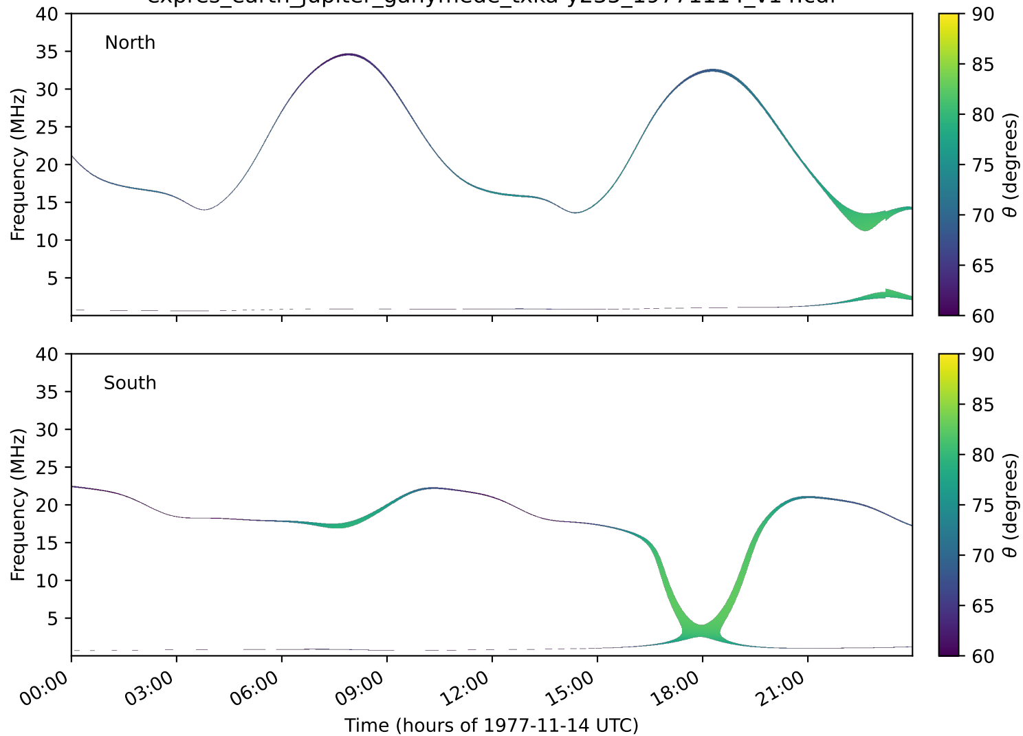
expres_earth_jupiter_ganymede_txka-y235_19771114_v14.cdf
