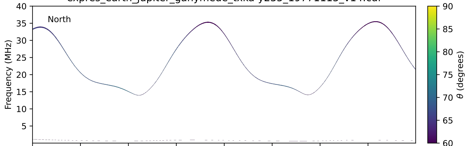
expres_earth_jupiter_ganymede_txka-y235_19771113_v14.cdf
