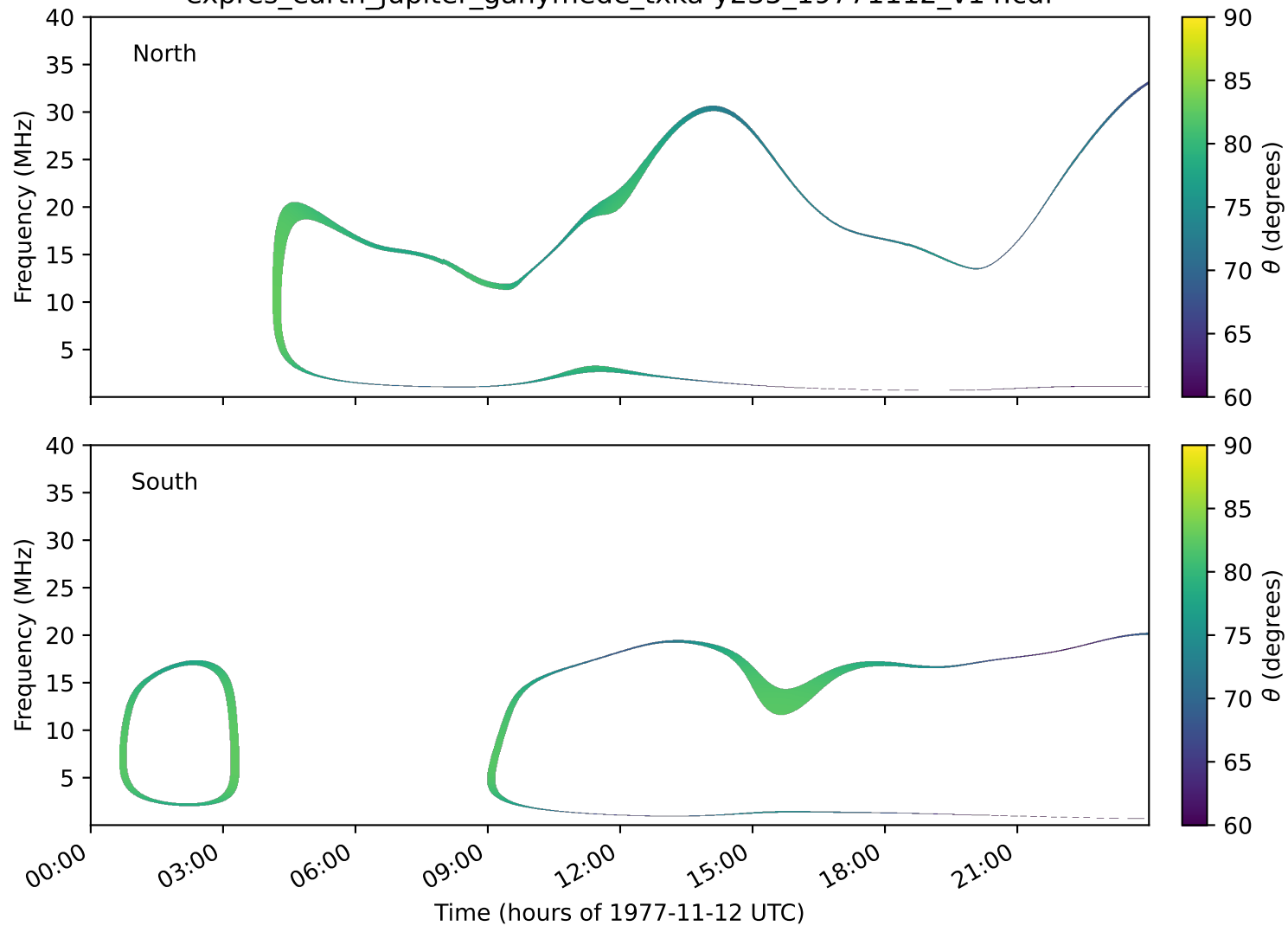
expres_earth_jupiter_ganymede_txka-y235_19771112_v14.cdf
