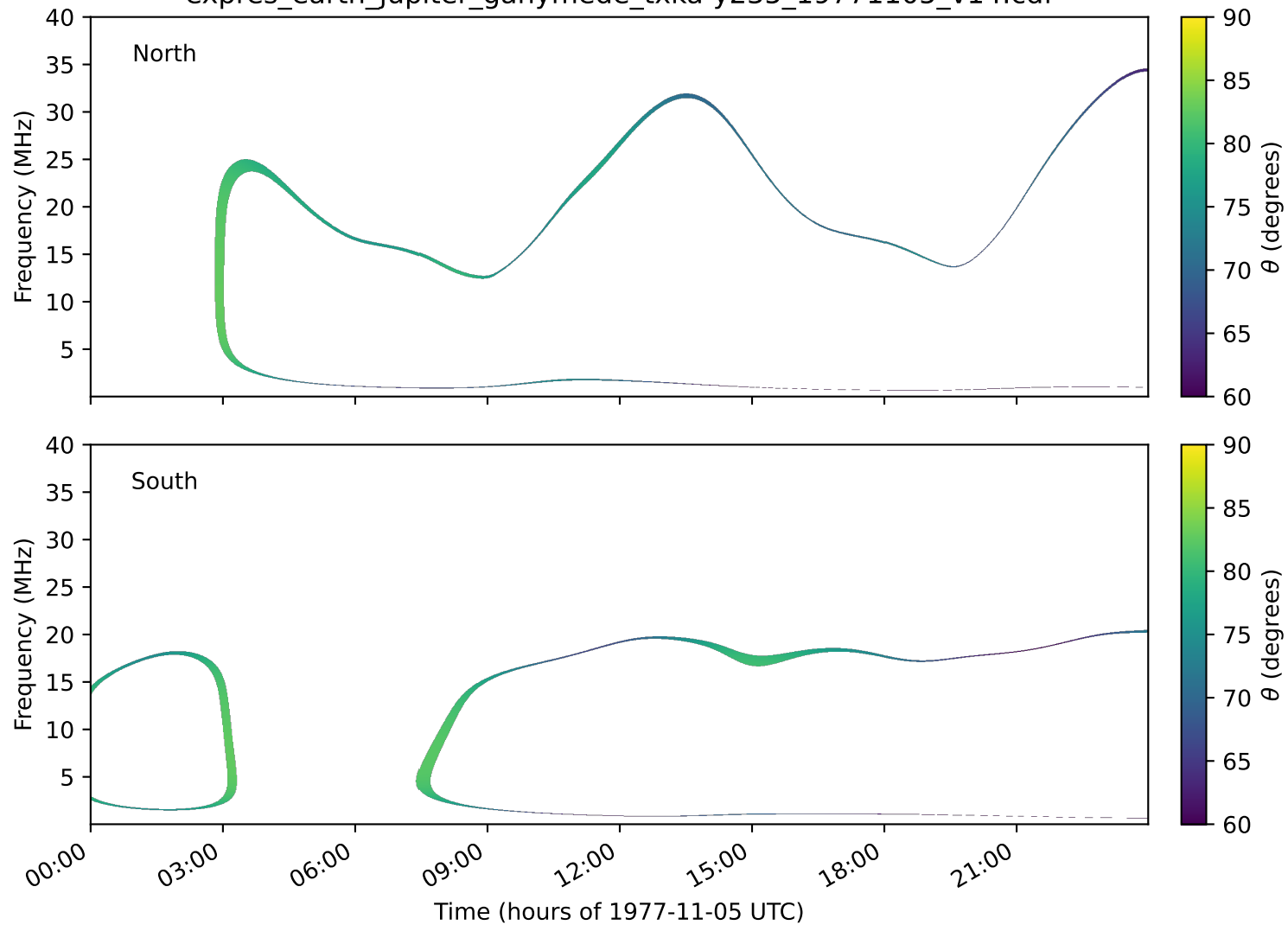
expres_earth_jupiter_ganymede_txka-y235_19771105_v14.cdf
