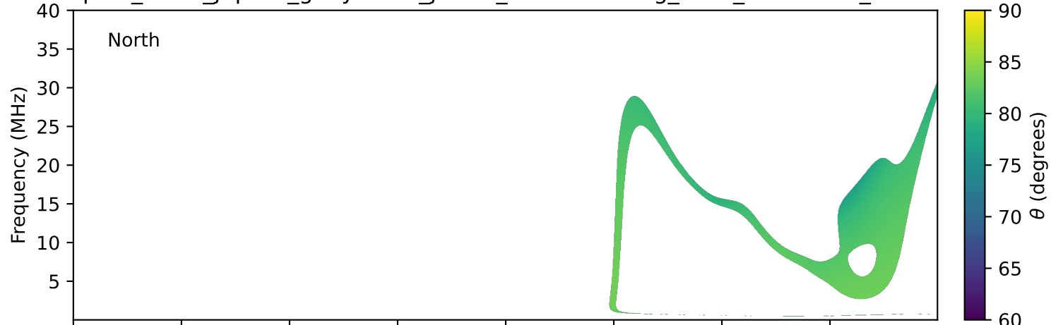
expres_earth_jupiter_ganymede_jrm33_lossc-wid1deg_3kev_19771126_v11.cdf
