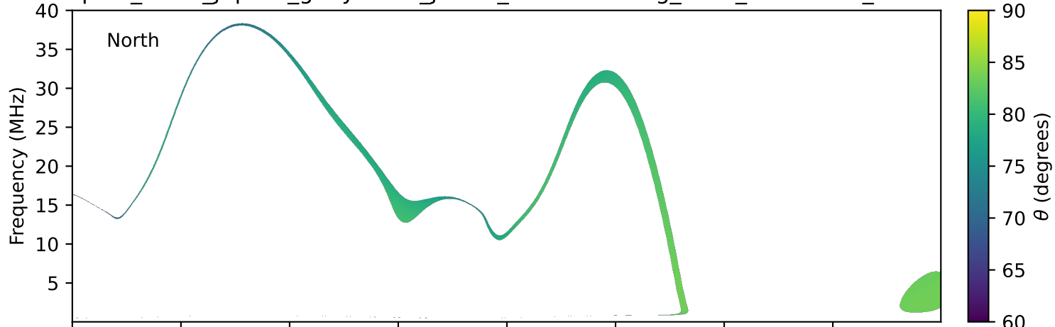
expres_earth_jupiter_ganymede_jrm09_lossc-wid1deg_3kev_19771122_v11.cdf
