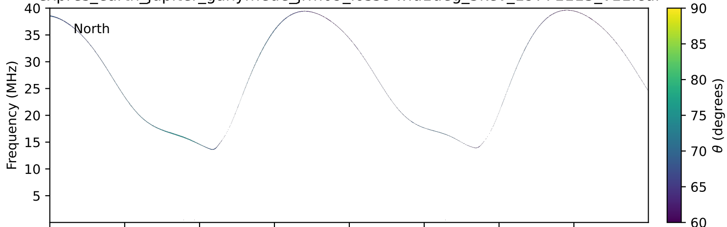
expres_earth_jupiter_ganymede_jrm09_lossc-wid1deg_3kev_19771113_v11.cdf
