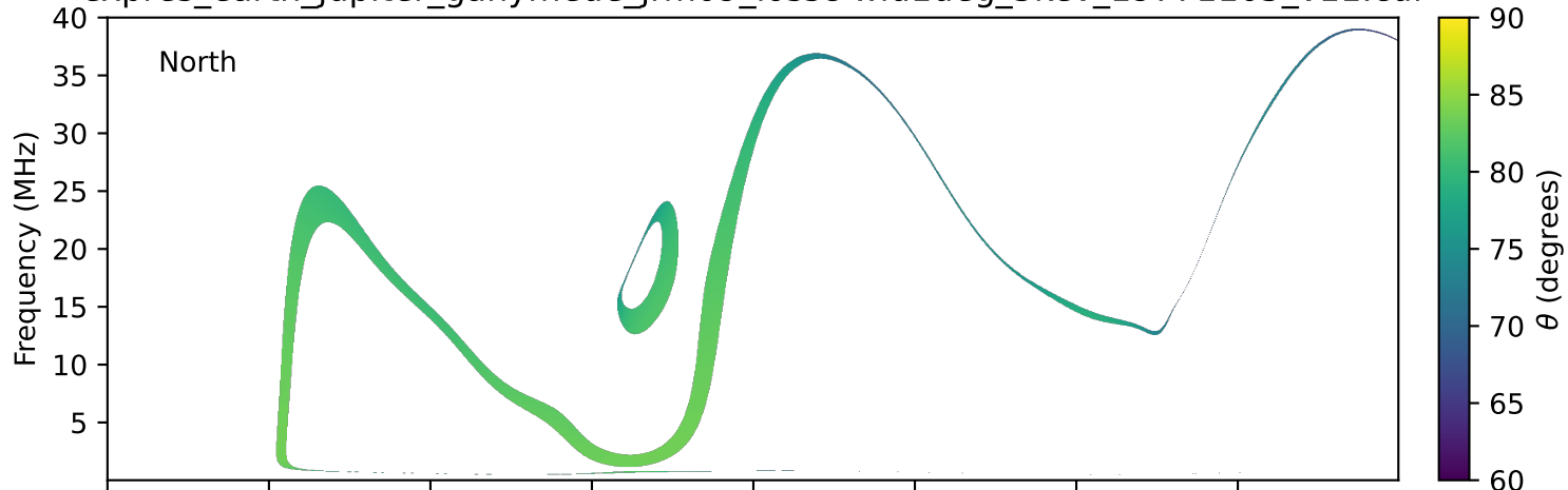
expres_earth_jupiter_ganymede_jrm09_lossc-wid1deg_3kev_19771105_v11.cdf
